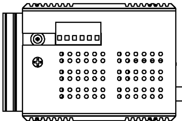
Figure 2.4: Top View of EKI-7529MI, EKI-7529MI/ST
