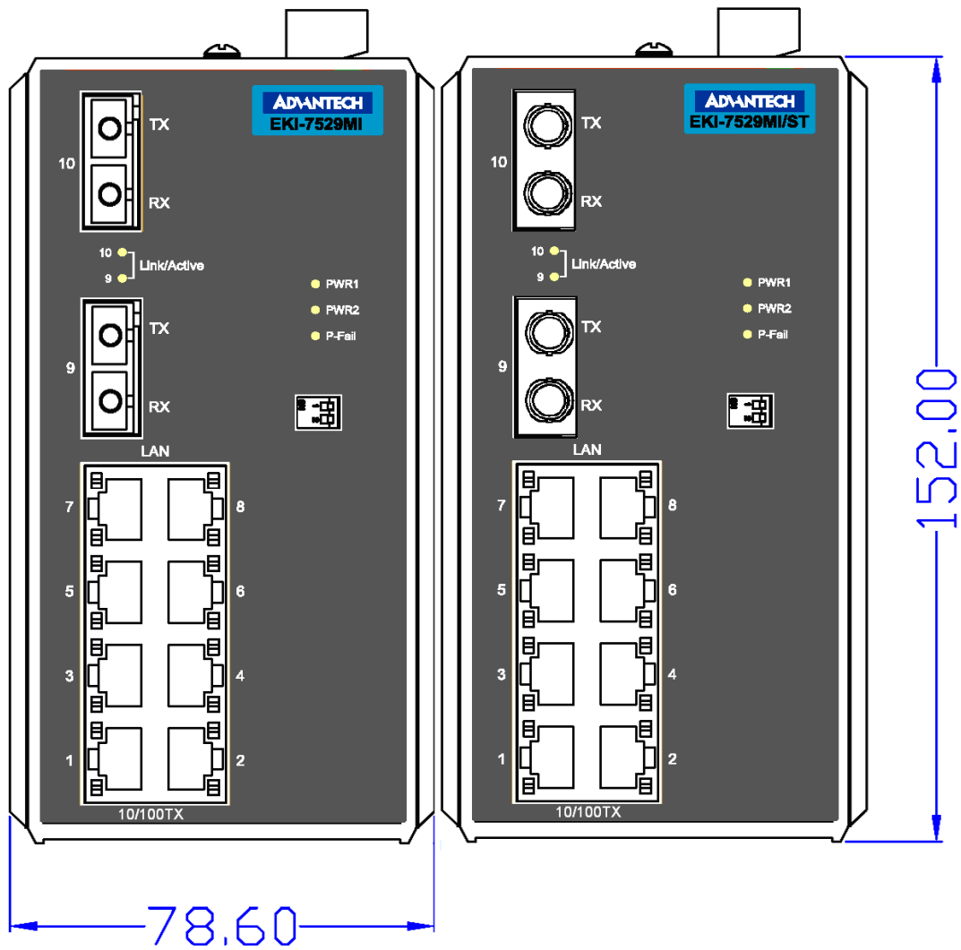
Figure 2.1: Front View of EKI-7529MI, EKI-7529MI/ST
