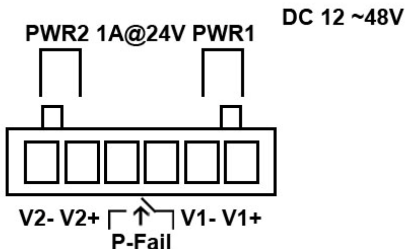
Figure 2.8: Pin Assignment of the Power Connector
