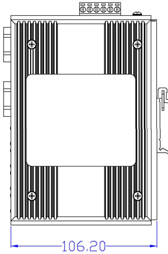
Figure 2.2: Side View of EKI-7529MI, EKI-7529MI/ST
