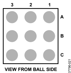
VIEW FROM BALL SIDE 07796-021 Figure 3. Pin Configuration
