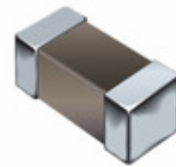
CS160808-R56K Bourns Inc. FIXED IND 560NH 150MA 900 MOHM
